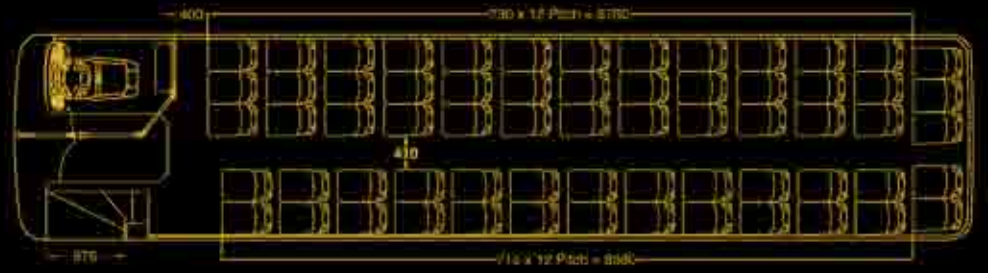
LAYOUT OF MCV S121R | 65 FIXED PASSENGER SEATS + DRIVER
