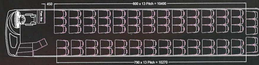
SEAT LAYOUT OF S140N 70 RECLINING PASSENGER SEATS + DRIVER
