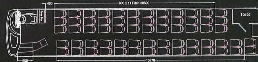
SEAT LAYOUT OF S140N 64 RECLINING PASSENGER SEATS + DRIVER
