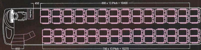
SEAT LAYOUT OF S140N 56 RECLINING PASSENGER SEATS + DRIVER
